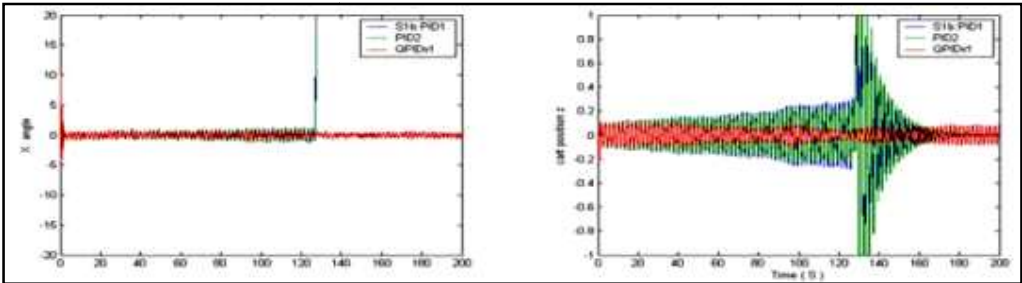
Figure 20. Pole motion (left) and cart motion (right) comparison in New 3 situation
