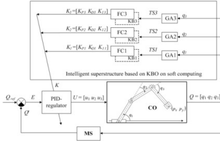
Figure 25. ICS with separated control based on KBO for 3DOF manipulator
