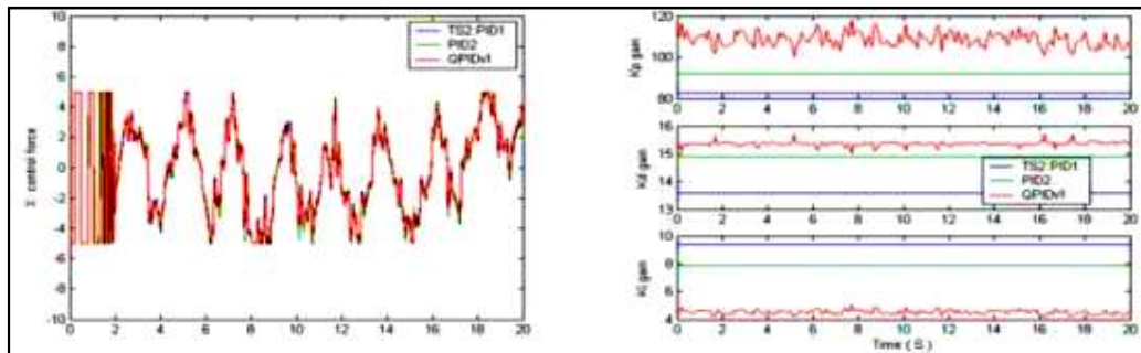
Figure 15. Control force and control laws in TS2 situation
