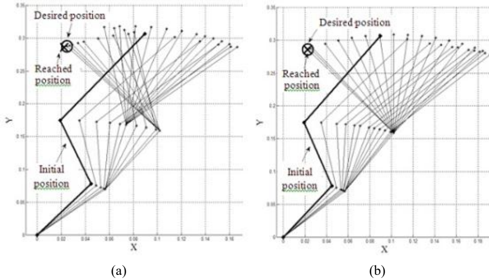
Figure33. ICS based on KBO on soft computing with one FC in the conditions of an internal unexpected control situation (a); ICS based on quantum computing (b)
