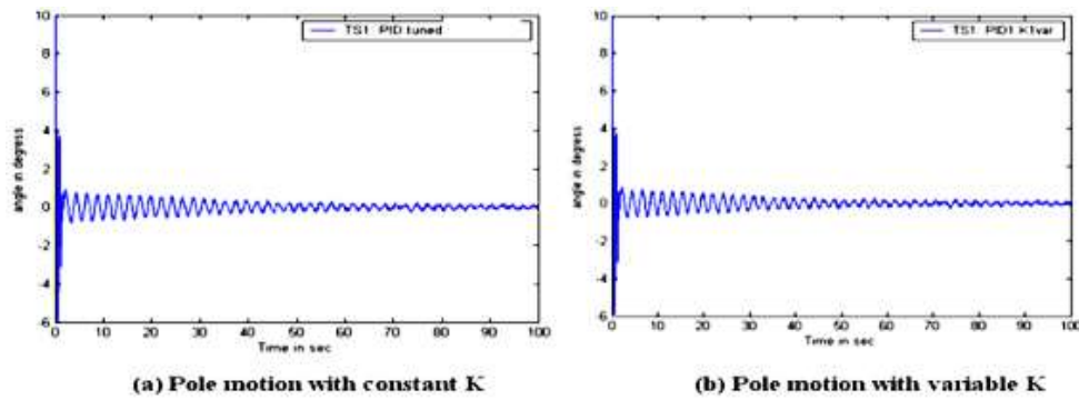
Figure4. Teaching conditions 1: Pole motion with constant and disturbed K -gains of PID1
