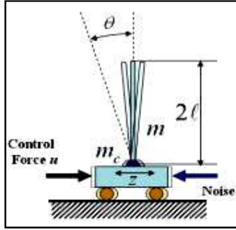
Figure2. Geometrical model of cart-pole system
