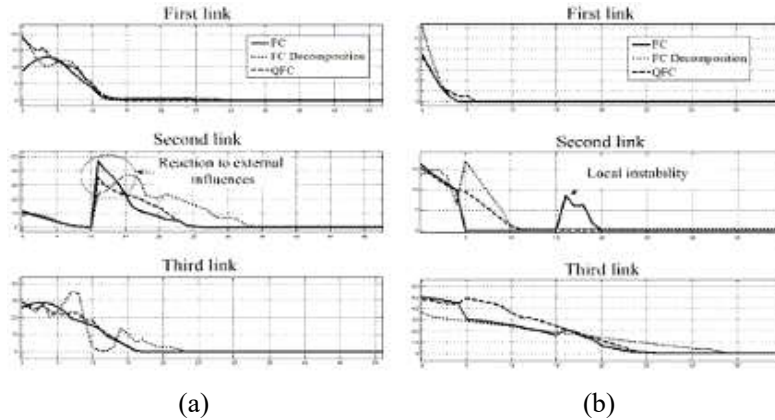
Figure 34. Control signals generated by different types of ICS in unexpected control situations
