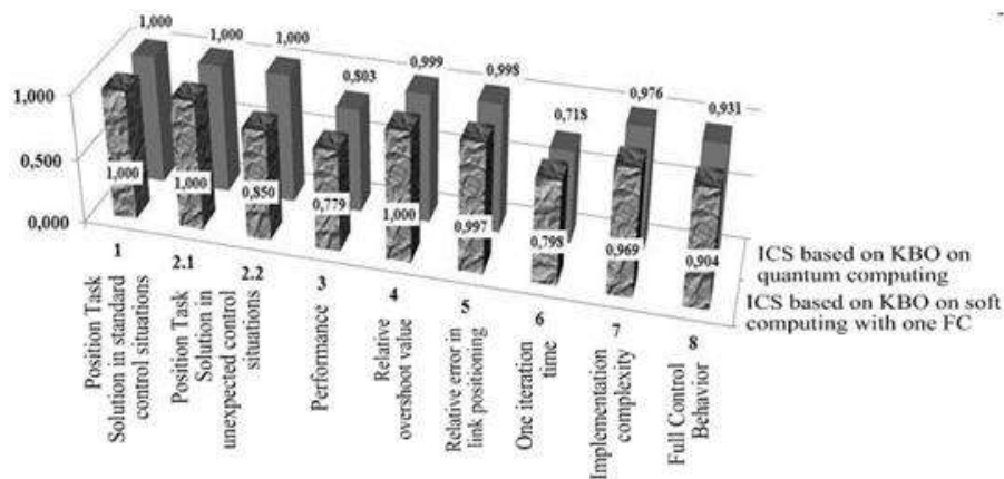
Figure 31. Comparison of the results of ICS based on KBO on soft computing with one FC and ICS based on quantum computing when testing Matlab / Simulink models
