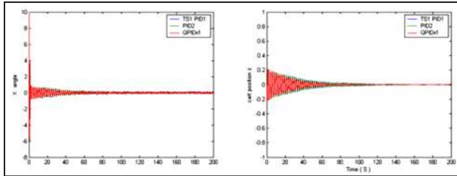
Figure12. Pole motion (left) and cart motion (right) comparison
