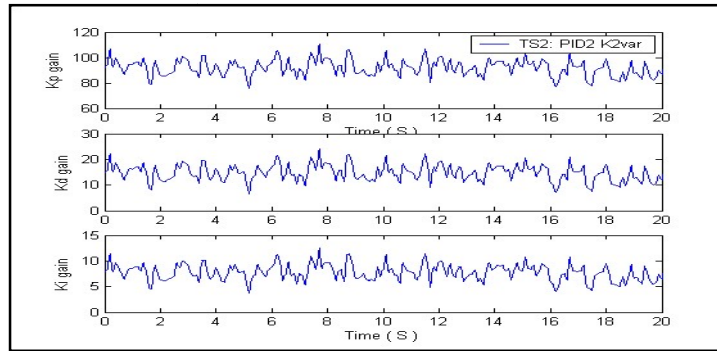
Figure7. Teaching conditions 2: Control laws
