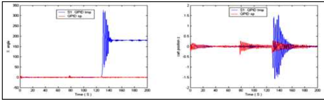
Figure 22. Pole motion (left) and cart motion (right) comparison in New 1 situation
