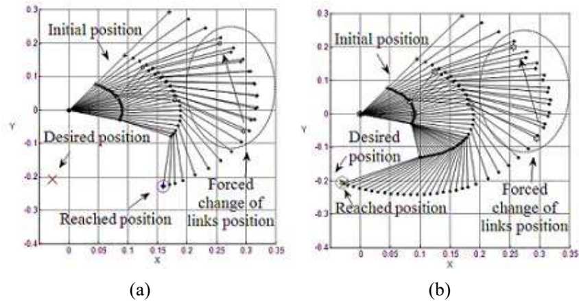
Figure 29. ICS based on KBO on soft computing with separated control in unexpected control situation (a); ICS based on KBO on quantum computing (b)
