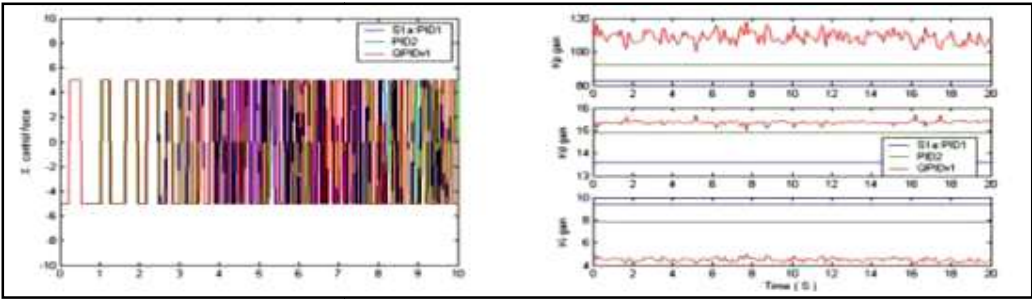
Figure 19. Control force and control laws in New 2 situation
