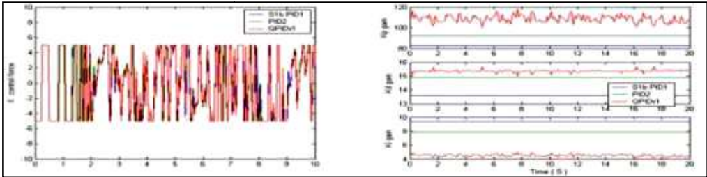
Figure 21. Control force and control laws in New 3 situation
