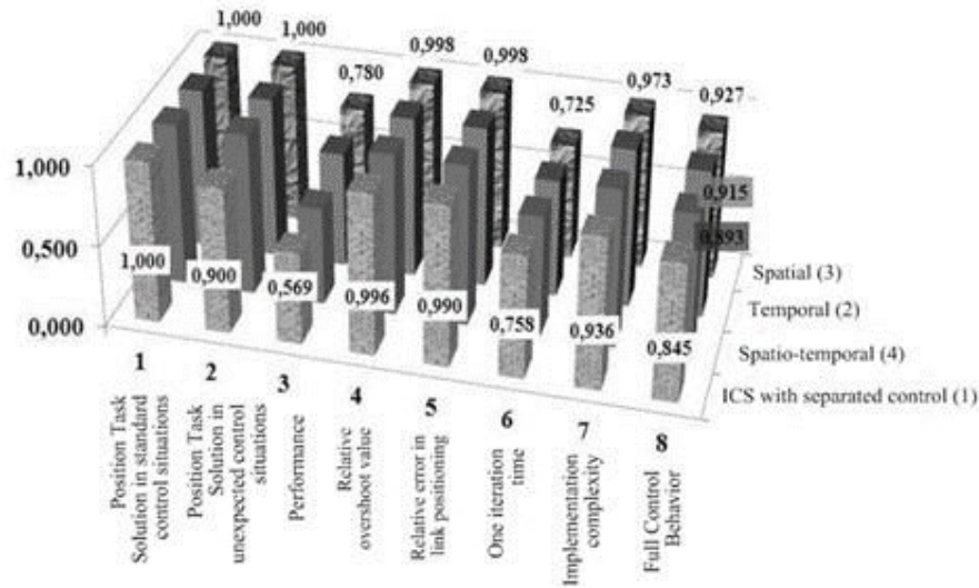
Figure28. Comparison of the results of ICS based on KBO on soft computing with separate control (1) and ICS based on quantum computing using temporal (2), spatial (3) and spatio-temporal (4) correlations when testing manipulator Testbench
