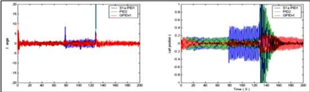
Figure 18. Pole motion (left) and cart motion (right) comparison in New 2 situation
