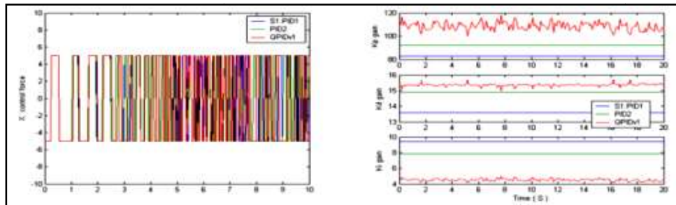
Figure 17. Control force and control laws in New 1 situation
