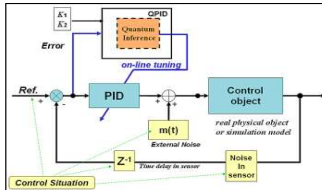
Figure 1. General structure of QPID based on two K-gains of classical PID and quantum inference
