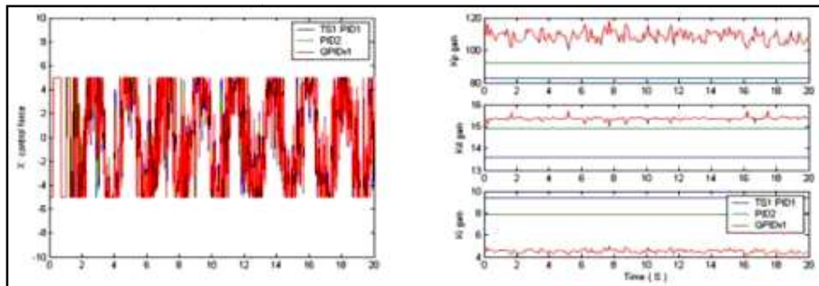
Figure 13. Control force and control laws
