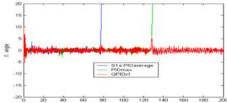
Figure 24. Pole motion under three types of control
