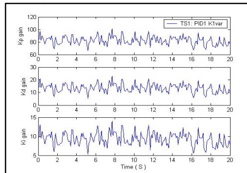
Figure5. Teaching conditions 1: Control laws
