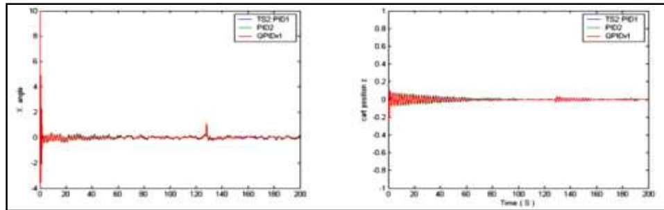
Figure 14. Pole motion (left) and cart motion (right) comparison in TS2 situation
