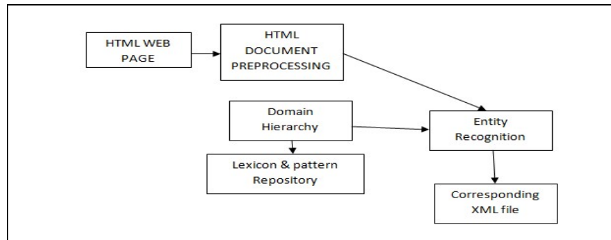
Figure.2. HTML to XML Conversion
