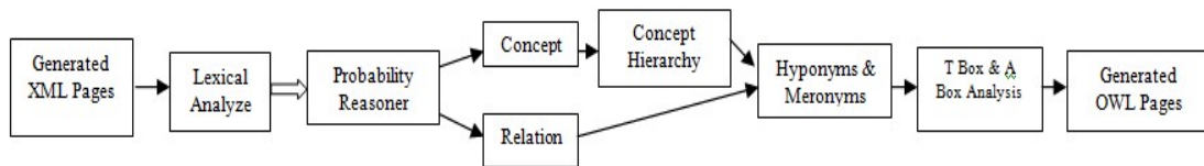
Figure 5. Semantic Analysis
