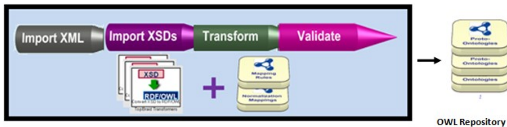
Figure 4. Syntactic Analysis
