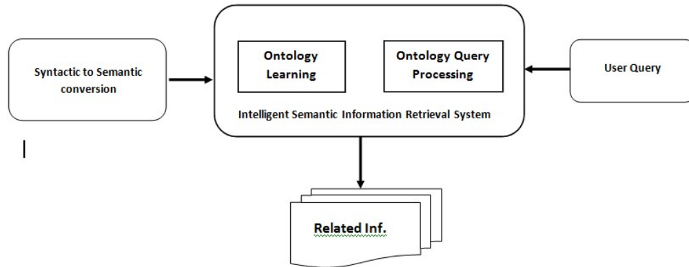
Figure 6. Intelligent Semantic Information Retrieval System
